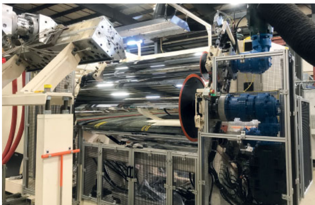
The new XP Express® – AGT rollstand for extrusion sheet and cast applications
